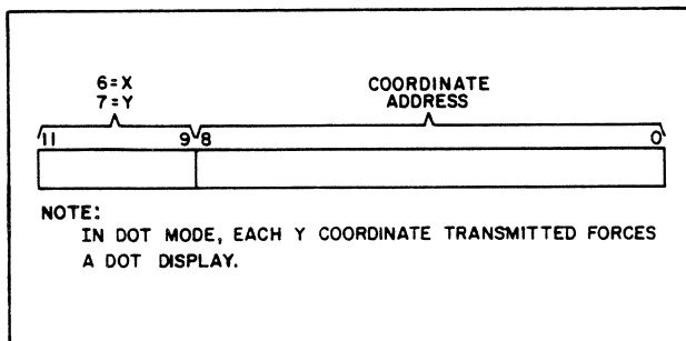
Figure 5-20. Coordinate Data Word
