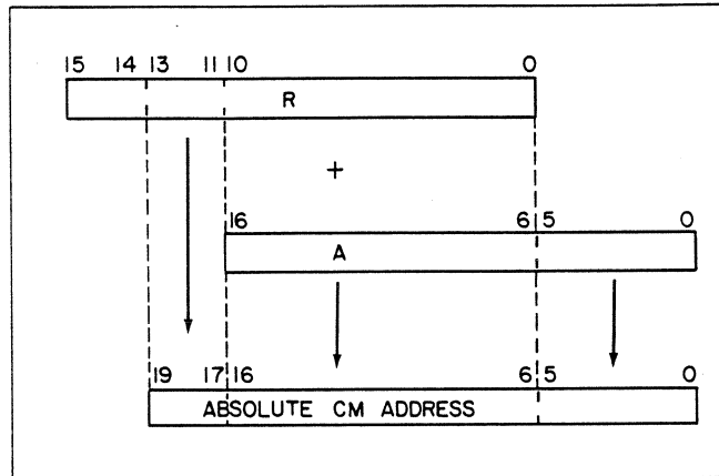
Figure 2-8. Formation of Absolute CM Address
