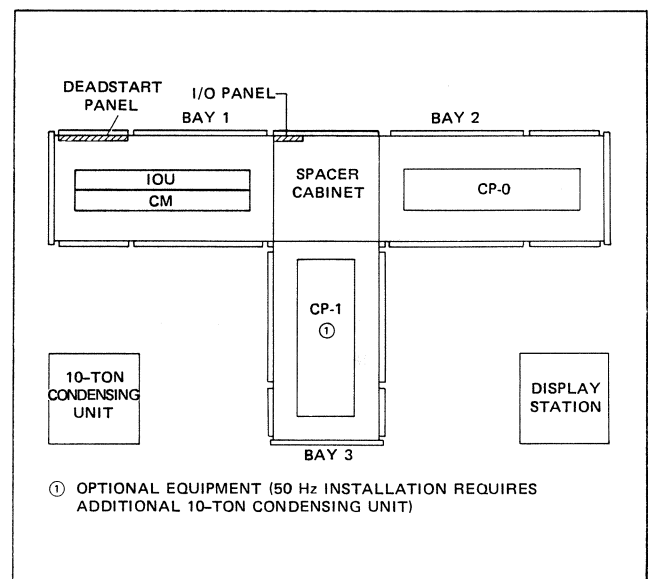
Figure 1-3. Model 865 Chassis Configuration (Top Cutaway View)
