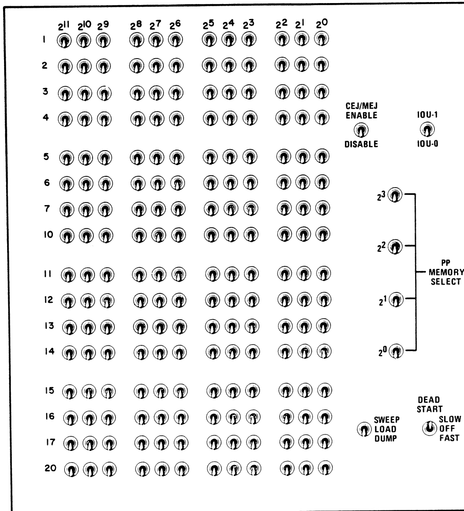
Figure 3-1. Deadstart Panel
