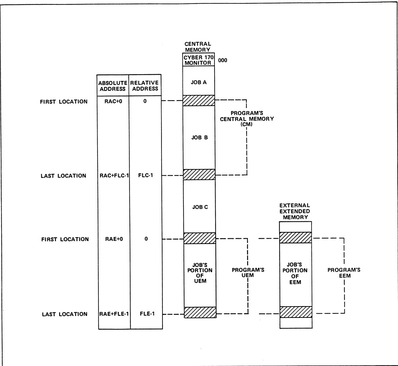
Figure 5-7. Memory Map
