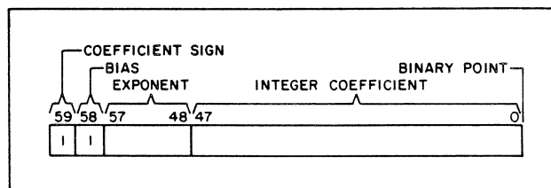
Figure 5-3. Floating-Point Format
