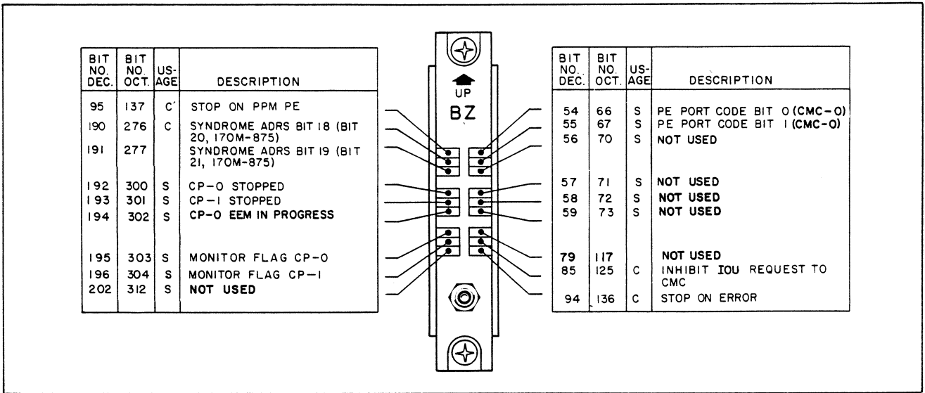
Figure 3-13. Module at 2C31
