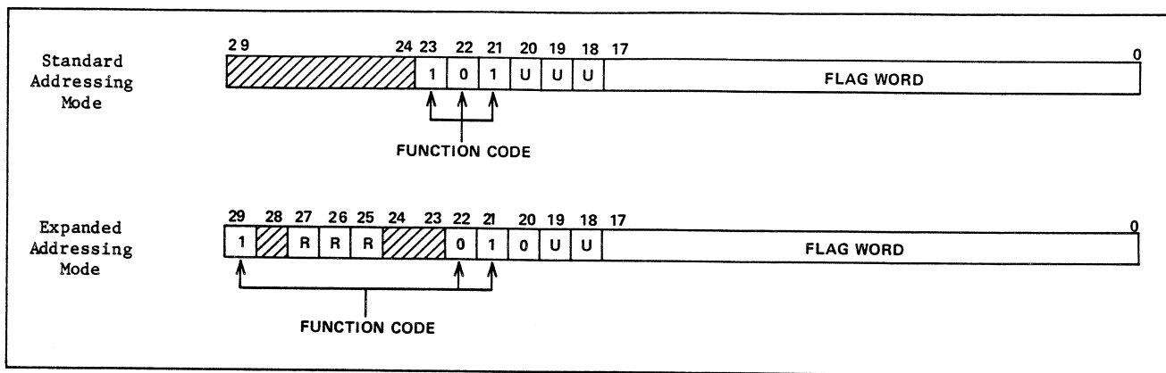
Figure 5-10. Selective Set Function Code
