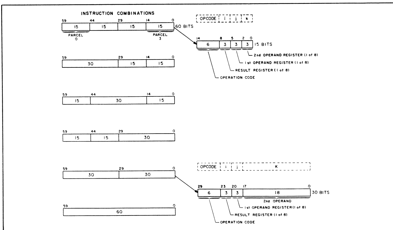
Figure 4-1. CP Instruction Parcel Arrangement
