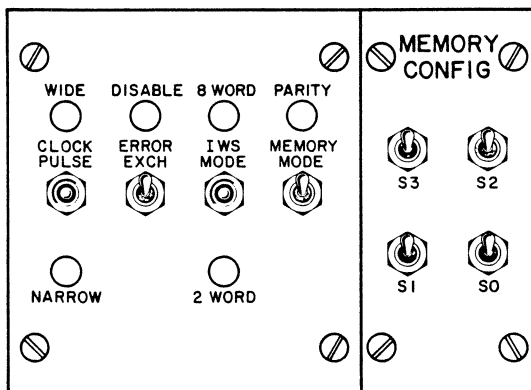
Figure 3-18. Modules 5A1 through 5A3
