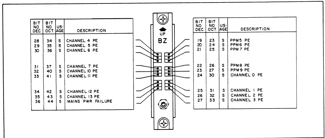
Figure 3-10. Module at 2D40
