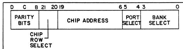
Figure 2-6. Model 170M-875 CM Address Format
