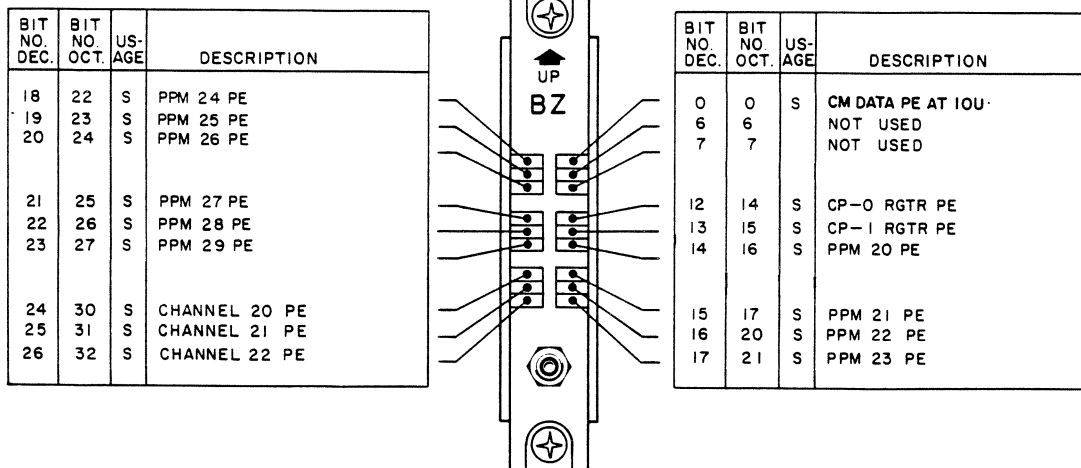
Figure 3-15. Module at 2N35
