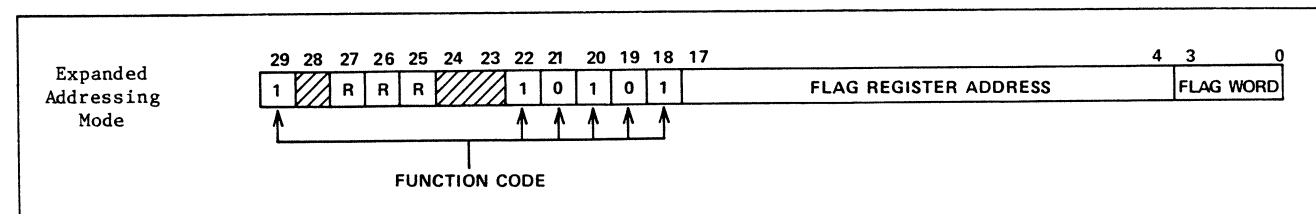
Figure 5-15. Detected Error Status Function Code
