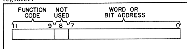
Figure 5-23. Descriptor Word
