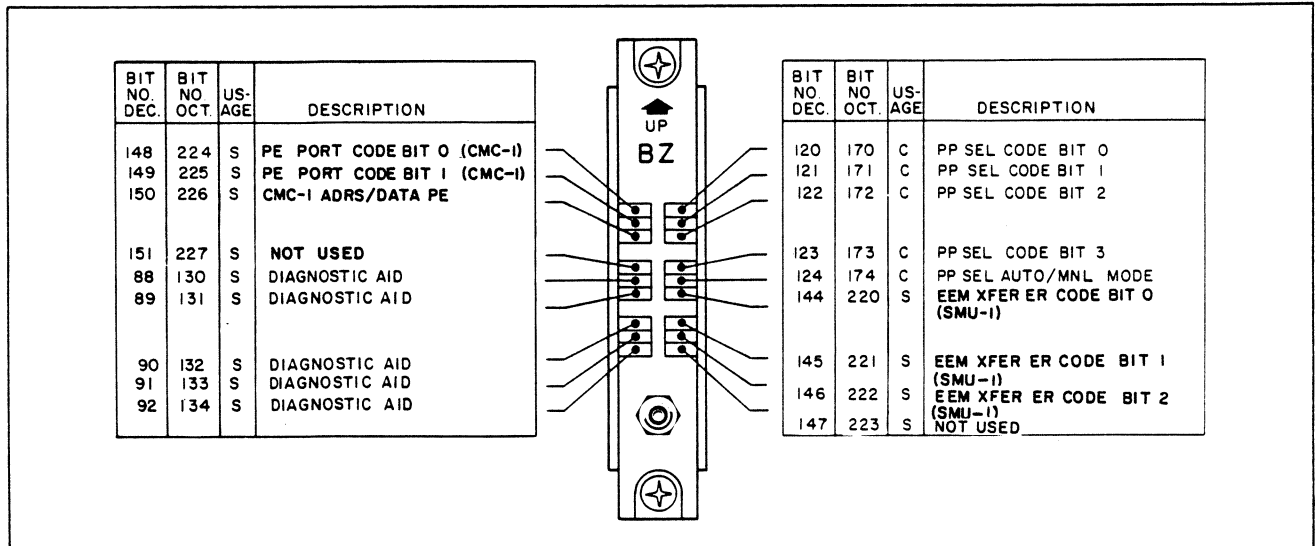
Figure 3-14. Module at 2E40
