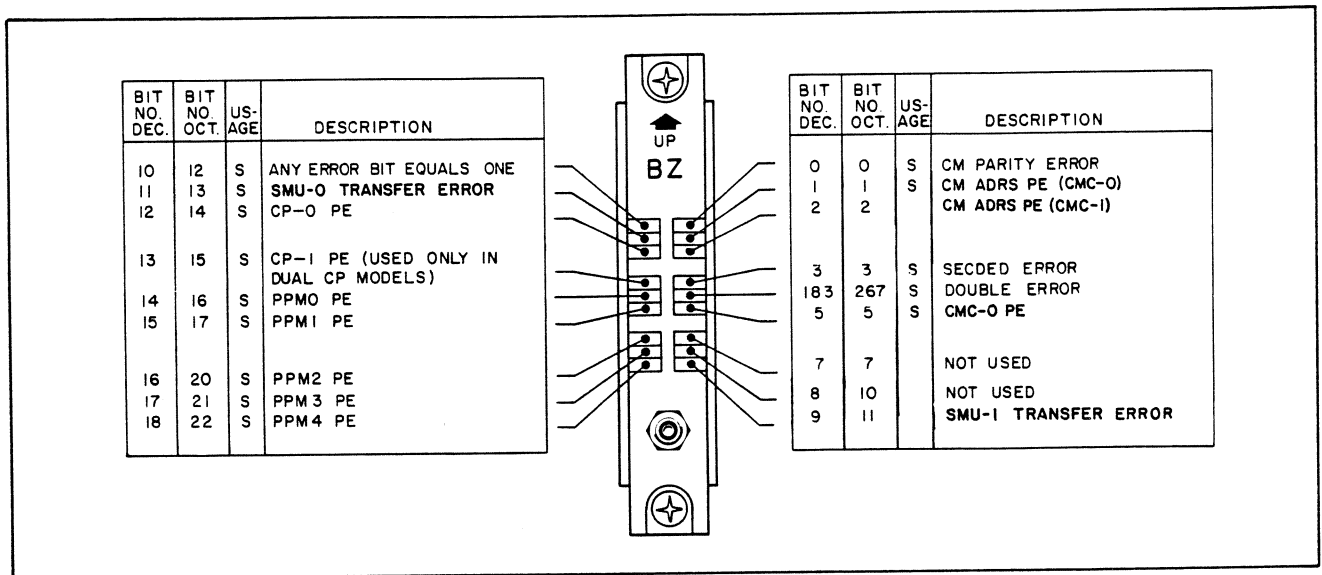
Figure 3-9. Module at 2C41
