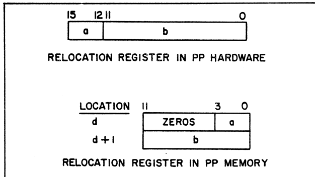
Figure 4-4. PP Relocation (R) Register Format
