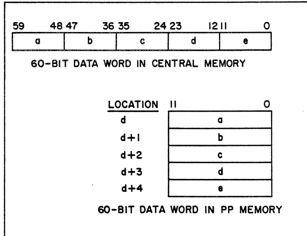
Figure 4-3. PP Data Format
