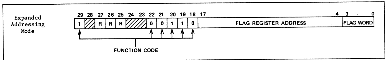
Figure 5-13. Zero/Select Function Code
