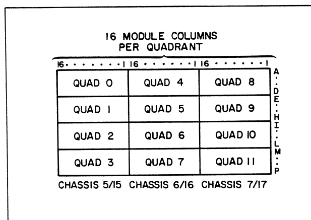
Figure 5-24. CP Chassis Quadrants (Viewed from Module Side)
