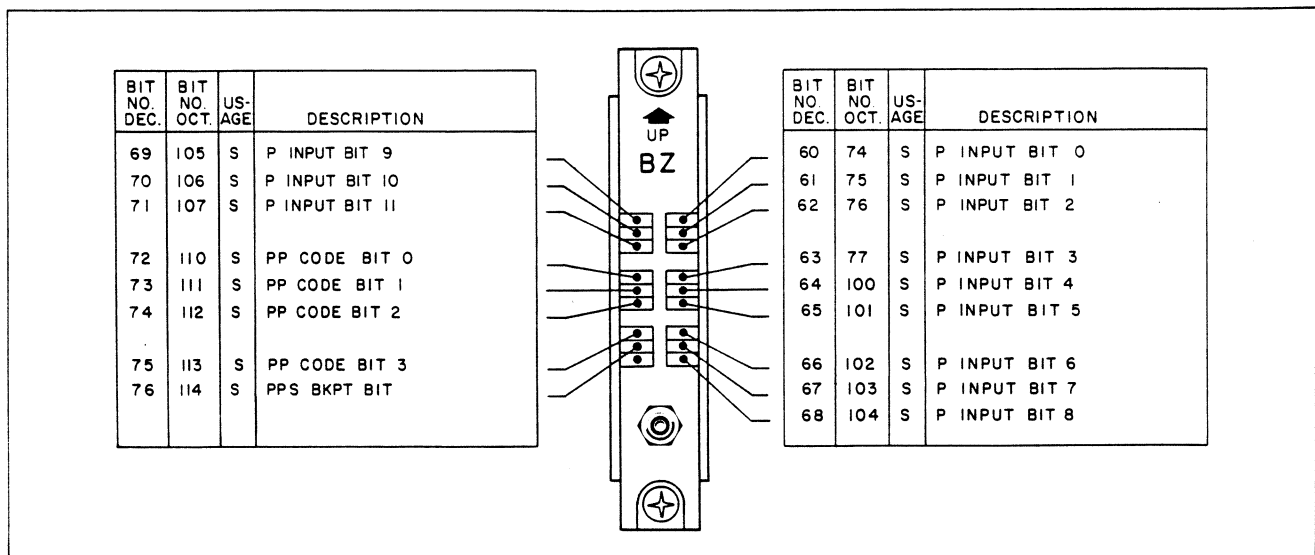
Figure 3-17. Module at 2P32
