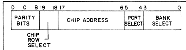
Figure 2-5. Model 875 CM Address Format
