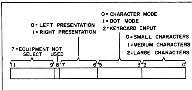
Figure 5-19. Display Station Output Function Code
