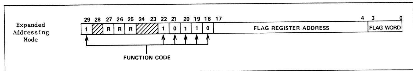
Figure 5-14. Equality Status Function Code
