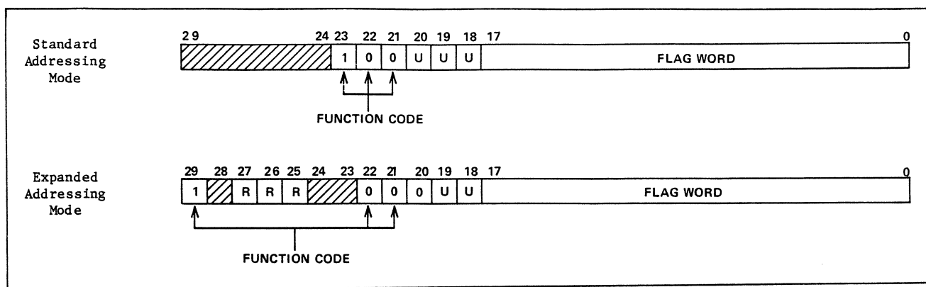
Figure 5-9. Ready/Select Function Code
