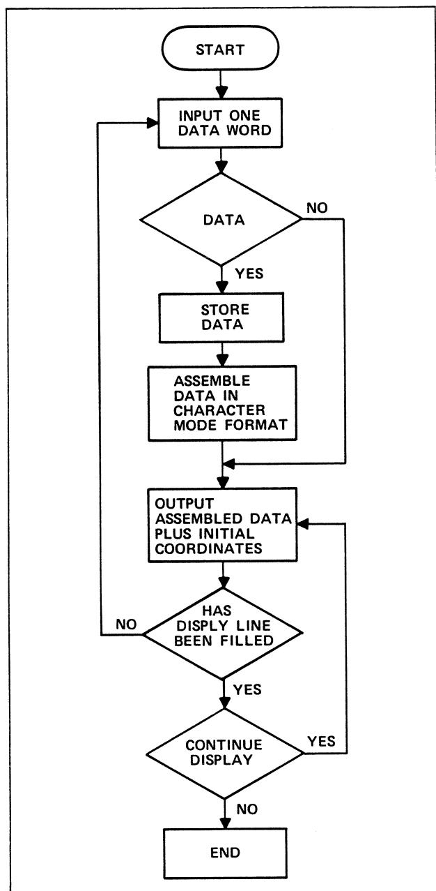
Figure 5-22. Receive and Display Program Flowchart
