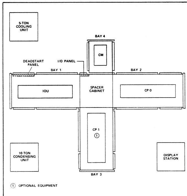
Figure 1-5. Model 170M-875 Chassis Configuration (Top Cutaway View)
