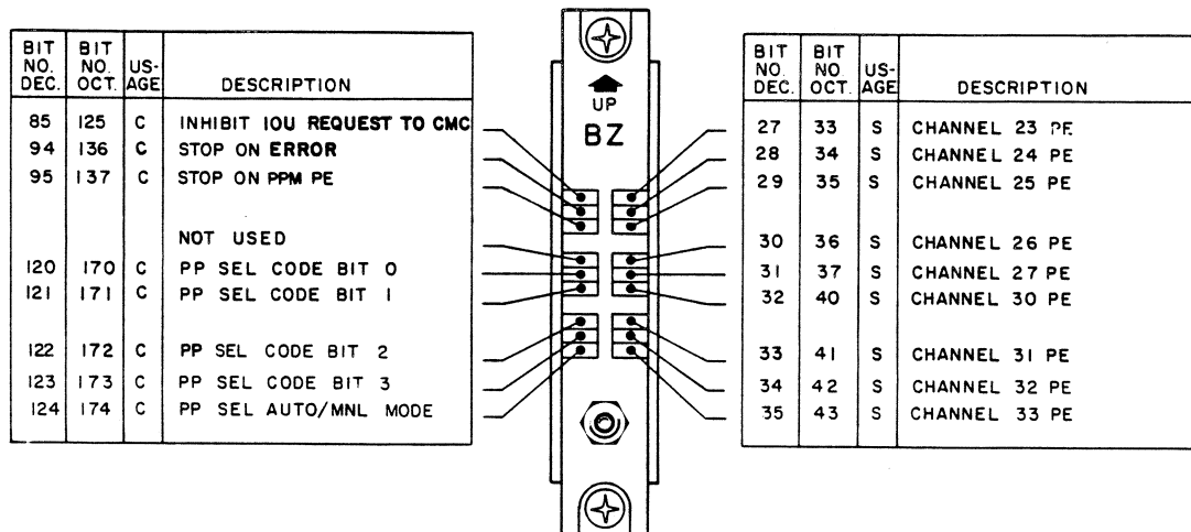
Figure 3-15. Module at 2N35
