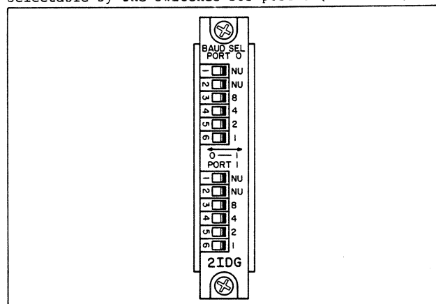
Figure 3-3. Module at 2P38
