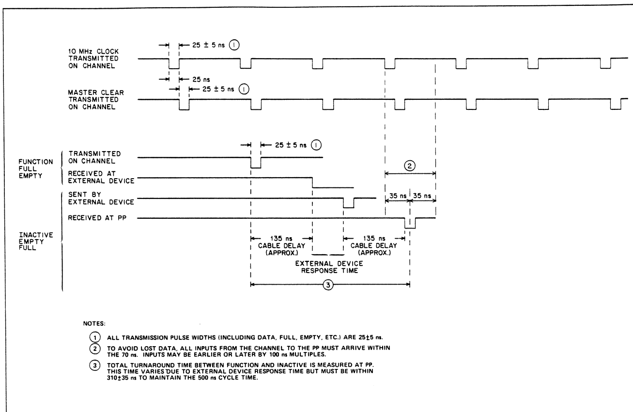
Figure 5-16. Channel Transfer Timing
