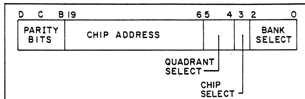
Figure 2-4. Model 865 CM Address Format
