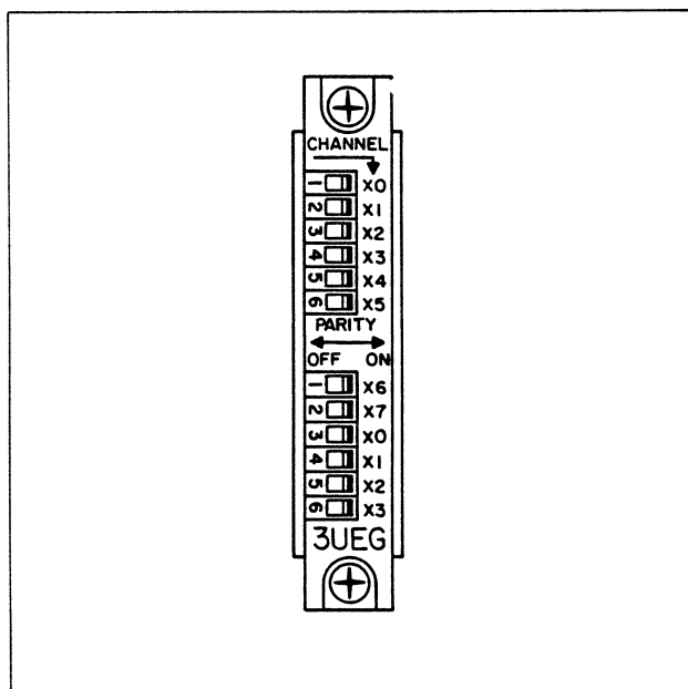
Figure 3-2. Module at I10 and J10
