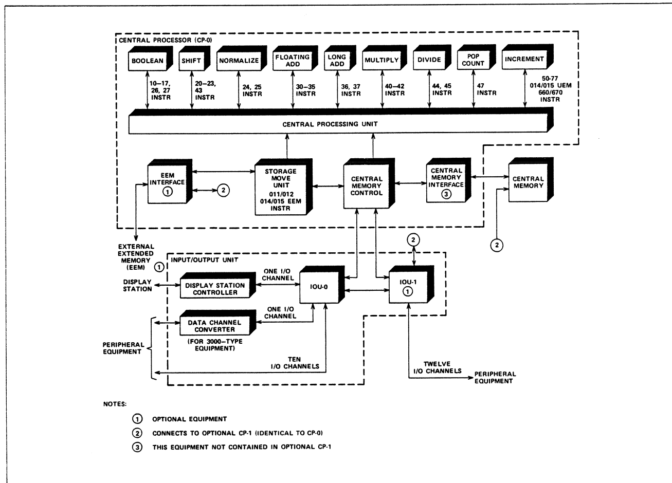
Figure 1-6. Models 865, 875, and 170M-875 - Block Diagram
