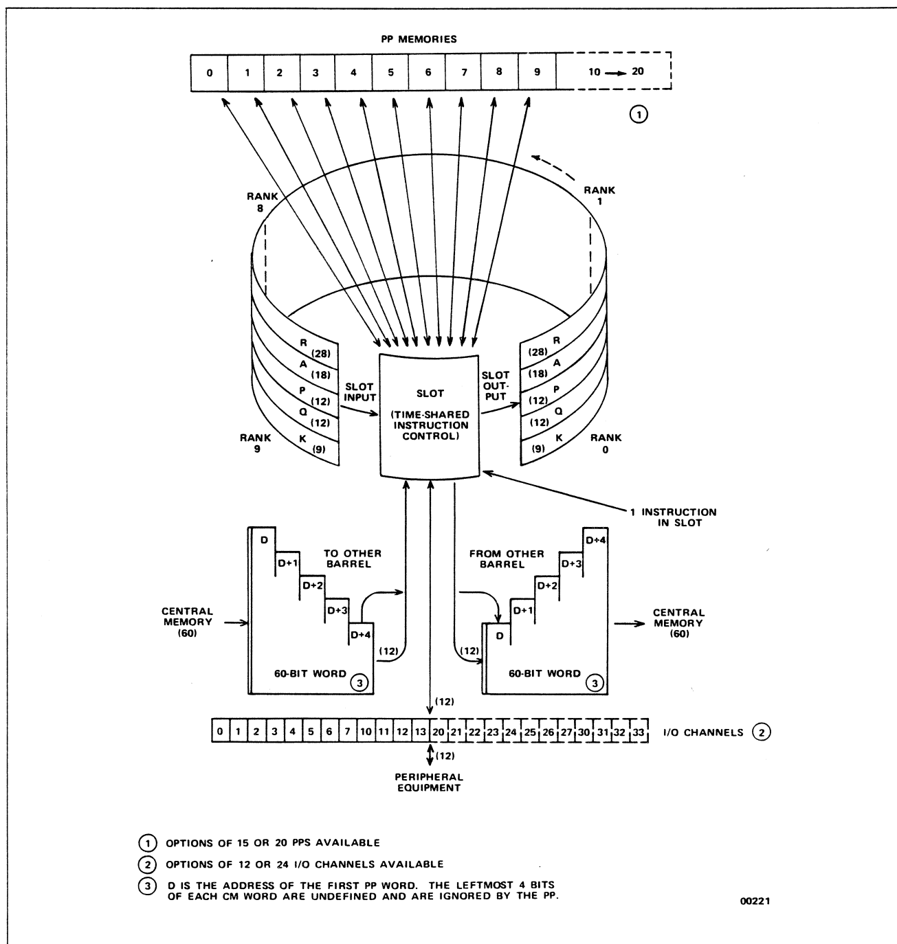
Figure 2-7. Barrel and Slot
