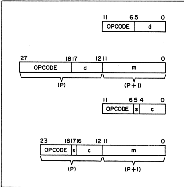
Figure 4-2. PP Instruction Formats
