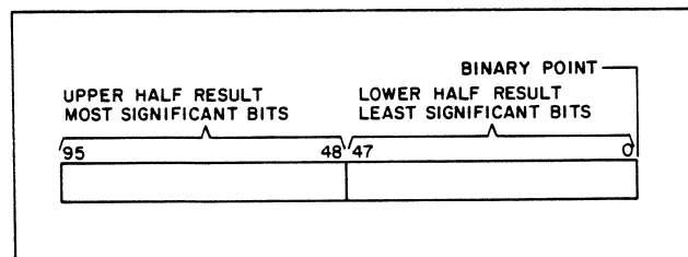
Figure 5-5. Multiply Result Format
