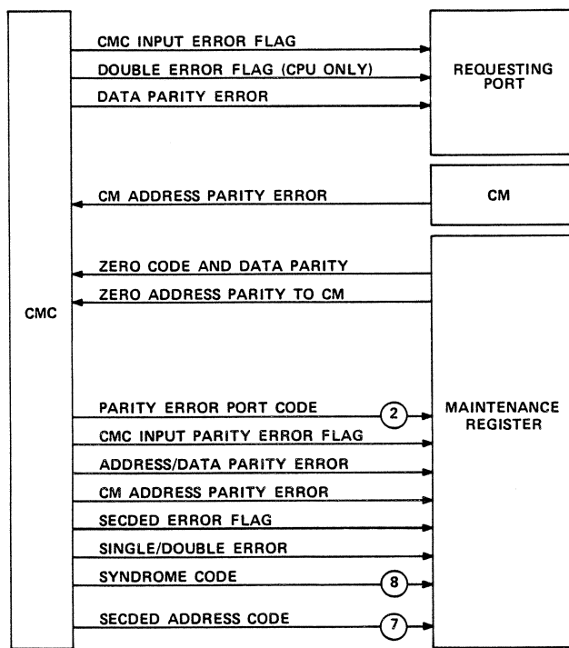
Figure 2-3. CMC Error Communications
