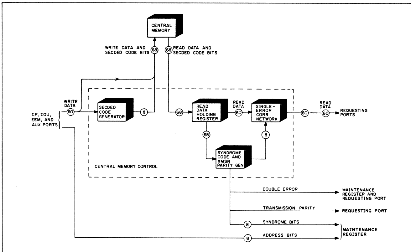
Figure 2-2. SECEDED Network Block Diagram (SECEDED Mode)
